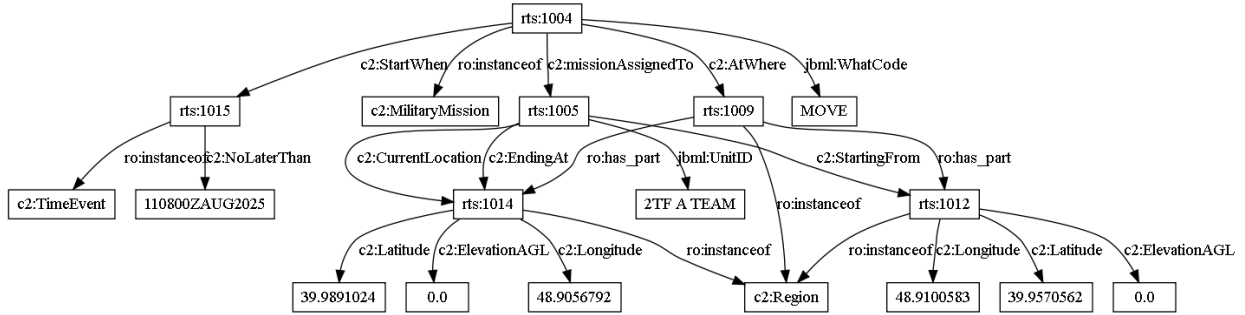
Fig. 3: Visualization of Ontologically Articulated Content of the XML message in Listing 1
