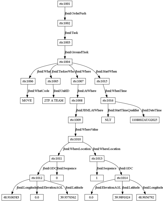
Fig. 2: Graph generated in the first step of the middleware
