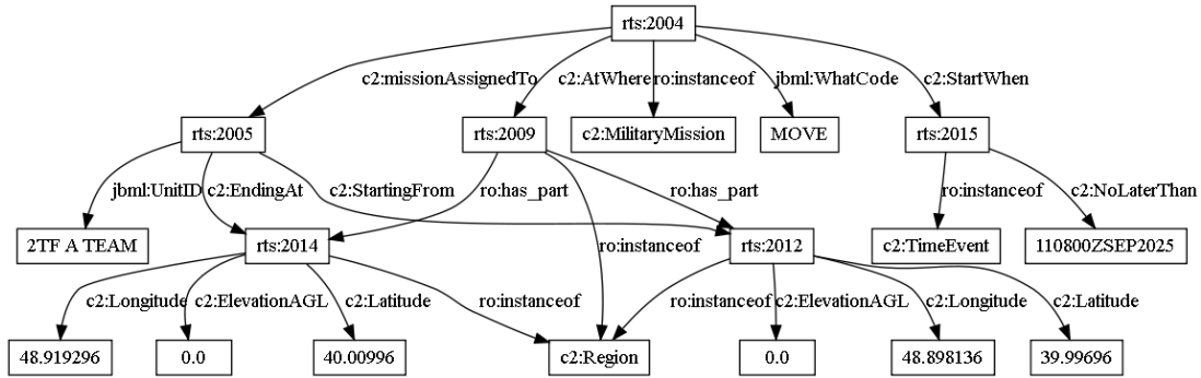
Fig. 4: Second Military Message after Processing via Step 2
