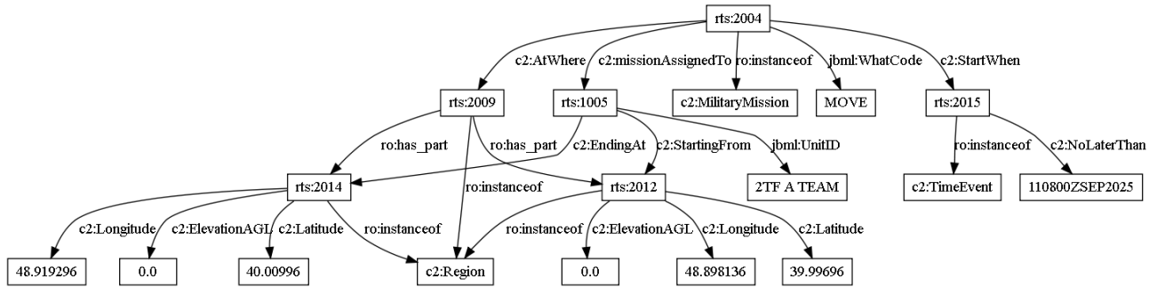
Fig. 5: Second Movement Mission as Described in the 2nd Example Message
