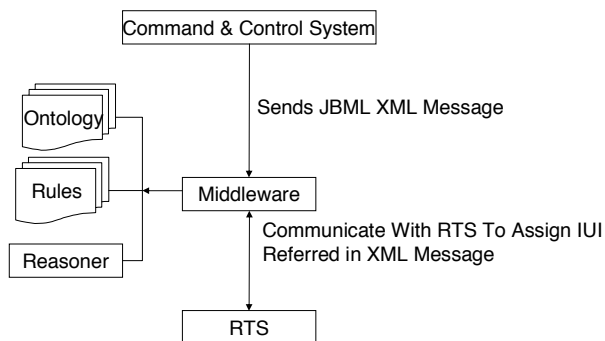
Fig. 1: Command & Control Application Integration with RTS
