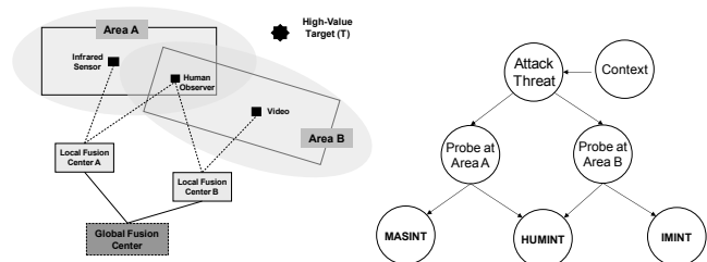
Figure 1: (left) An example distributed fusion environment; (right) A centralized BN model for situation assessment
