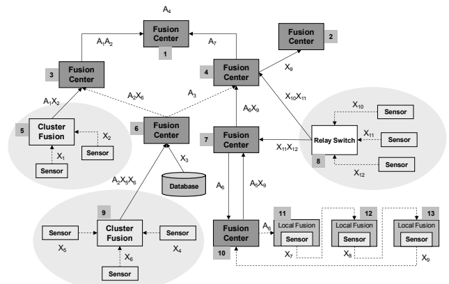
Figure 5: A typical distributed fusion environment
