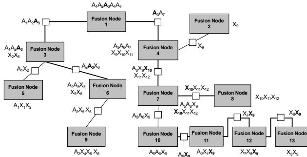
Figure 7: A junction tree from the distributed fusion environment
