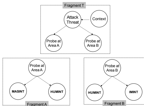
Figure 2: Distributed parts of the BN models
