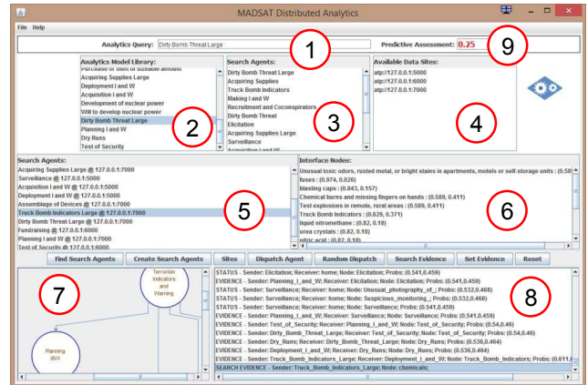
Figure 4: Distributed analytics interface
