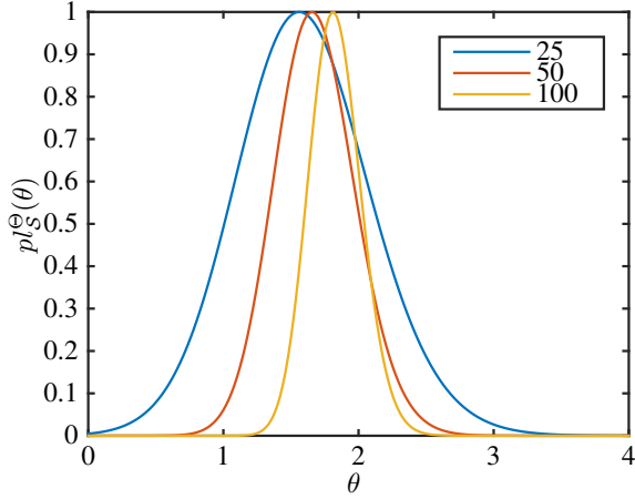
Fig. 1. Normalized likelihood function for different sample sizes.
