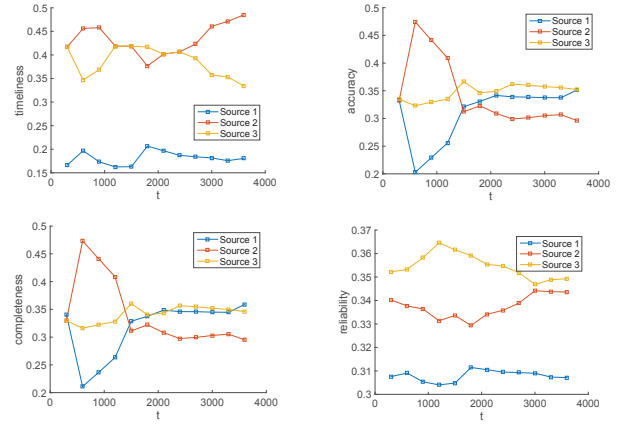
Fig. 5. QoI criteria scores for three sources based on AHP with (UL) Timeliness - T, (UR) Accuracy - A, (LL) Completeness - C, and (LR) Reliability - R.
