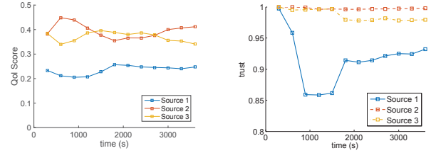
Fig. 6. QoI (L) and Trust (R) scores for the example scenario
