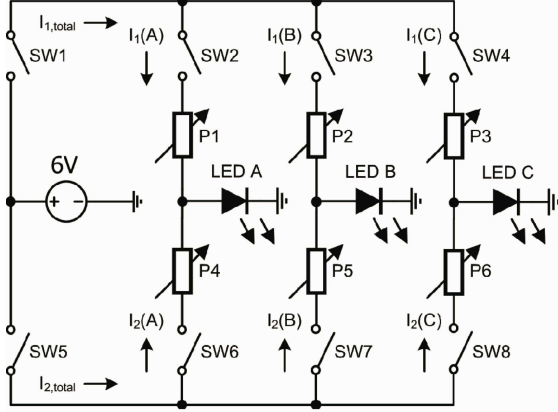
Figure 1. Z-box Scheme.
